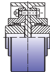
BRAKE DRUM GEAR COUPLING
