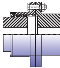
PAPER REFINER GEAR COUPLING
