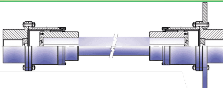
SLIDING TYPE GEAR COUPLING WITH BRAKE DISC
