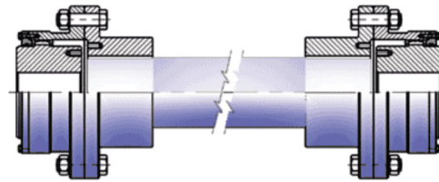
FLOAT SHAFT TYPE GEAR COUPLING RIGID IN SHAFT
